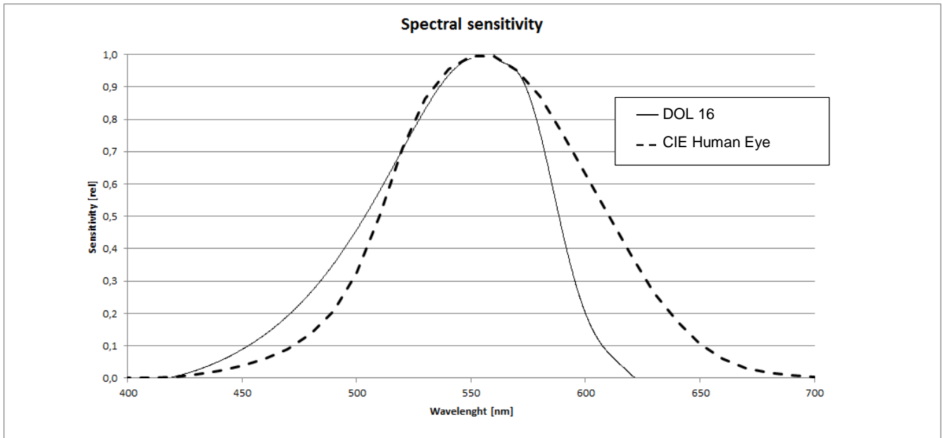
Figure 5: Spectral sensitivity
