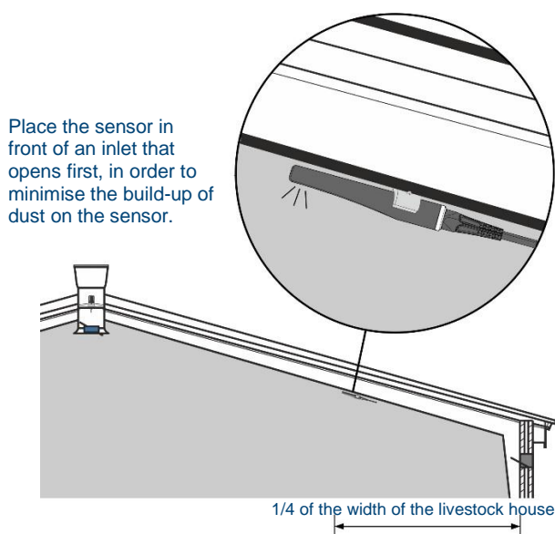
Figure 2: Mounting
