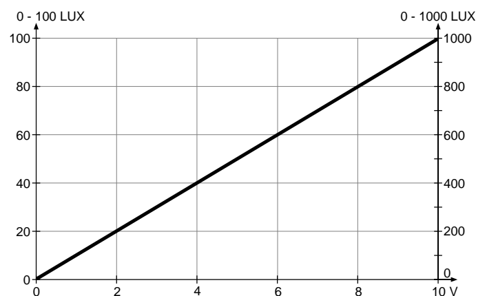
Output Voltage
